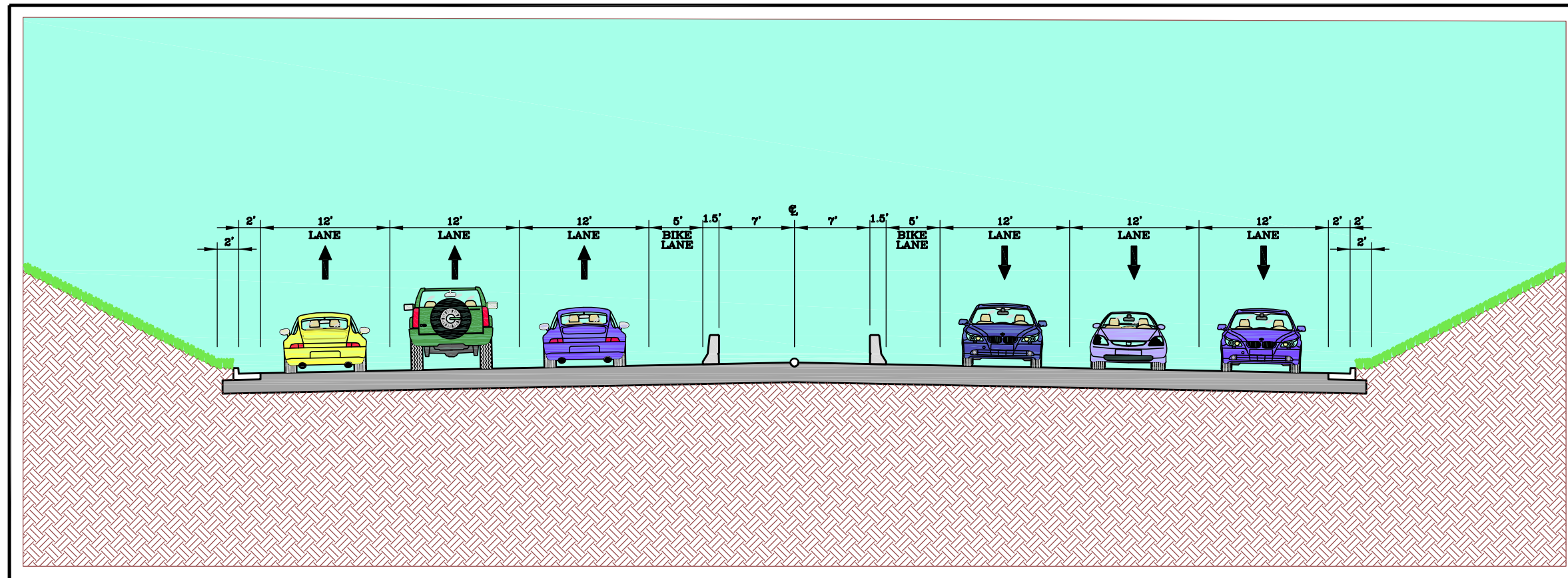
LEESTOWN ROAD DOUBLE CROSSOVER DIAMOND INTERCHANGE UNDER NEW CIRCLE ROAD BRIDGE
